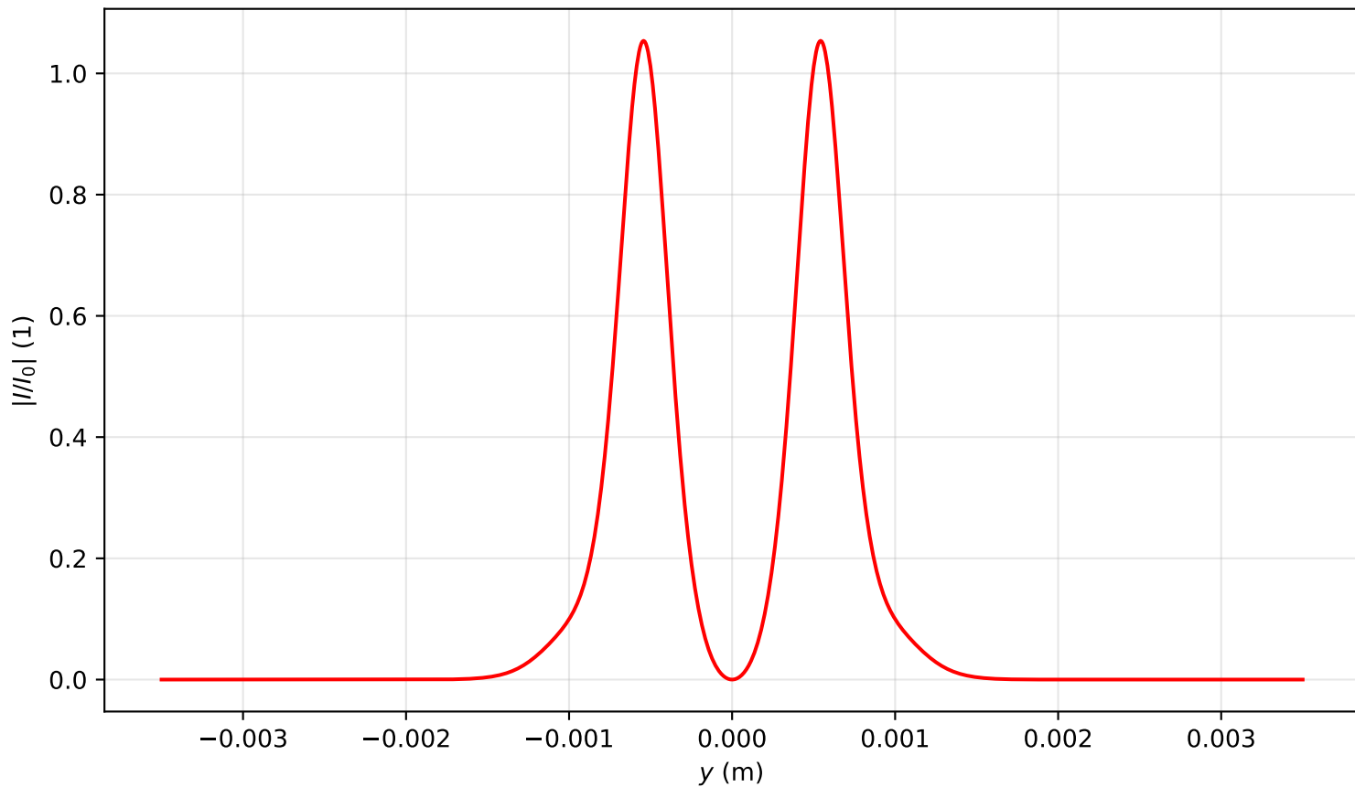
Intensity profile I(x=0, y, z=0.637)/I_0 , P_{in}=5.0P_{cr} , artificial time
